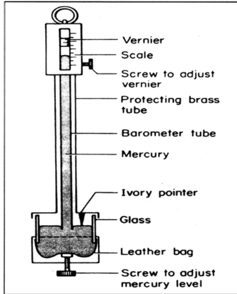
Fig. 2.6 Fortin Barometer
