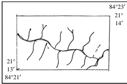
Parallel Drainage Pattern
